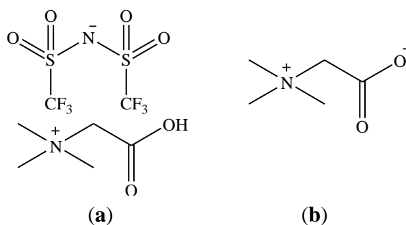
Figure 1. (a) Structure of the ionic liquid [Hbet][Tf_2N] ; and (b) The extracting agent betaine.
