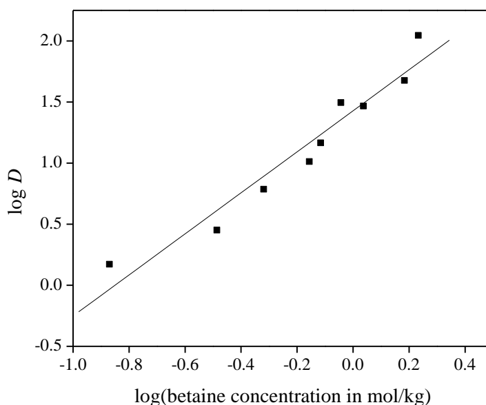
Figure 9. Slope analysis for the extraction of \text{Nd}(\text{Tf}_2\text{N})_3 in [\text{Hbet}][\text{Tf}_2\text{N}]-\text{H}_2\text{O} with zwitterionic betaine as extractant. Slope of linear fit is equal to 1.68 \pm 0.16 , the R -value of the fit is 0.97.
