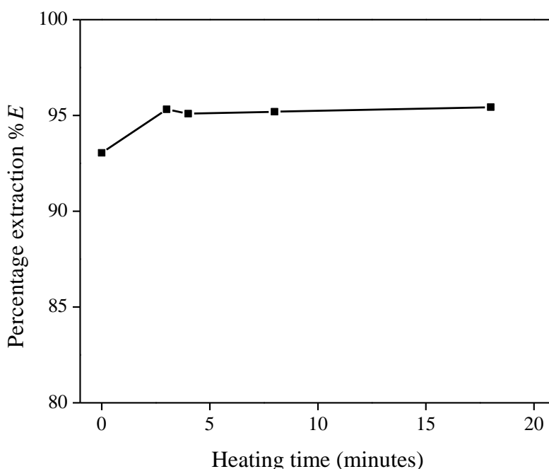
Figure 3. Percentage extraction (% E ) as a function of the heating time (in minutes) above the UCST, for the extraction of \text{Nd}(\text{Tf}_2\text{N})_3 in [\text{Hbet}][\text{Tf}_2\text{N}]-\text{H}_2\text{O} with betaine as extractant.
