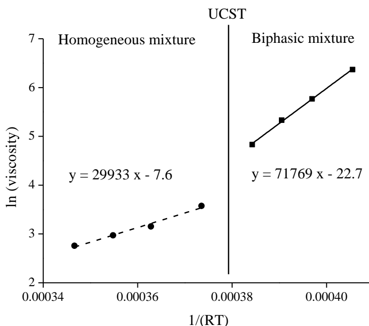
Figure 2. Arrhenius plot for [Hbet][Tf 2 N] in equilibrium above and under the upper critical solution temperature (UCST) with 53 wt % water containing the betaine extractant.
