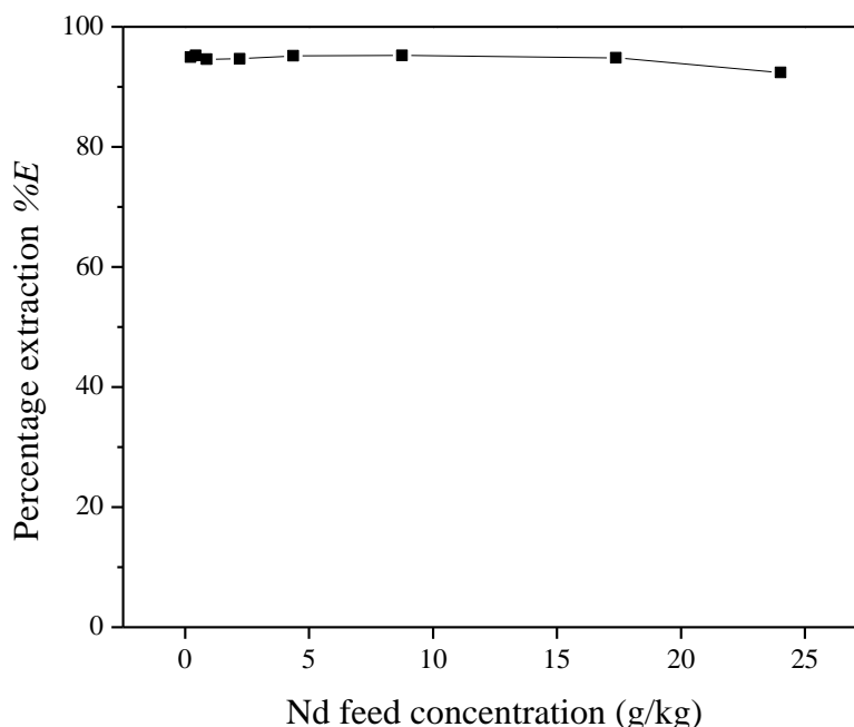
Figure 11. Percentage extraction (% E ) as a function of the neodymium feed concentration for the extraction of \text{Nd}(\text{Tf}_2\text{N})_3 in water-saturated [\text{Hbet}][\text{Tf}_2\text{N}] with zwitterionic betaine as the extractant.
