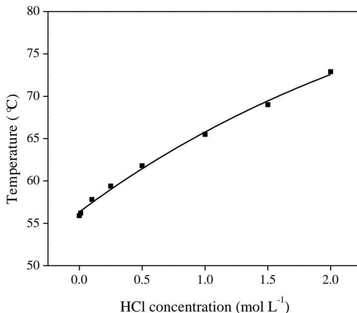
Figure 15. Influence of the HCl concentration in the aqueous phase on the cloud point of the [Hbet][Tf 2 N]–water mixture (50/50 wt % [Hbet][Tf 2 N] sat /H 2 O).
