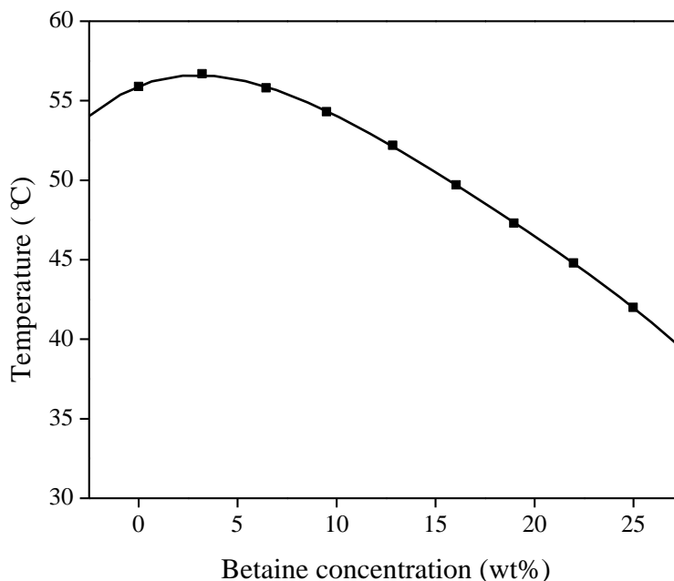
Figure 14. Influence of the betaine concentration in the aqueous phase on the cloud point of a [Hbet][Tf 2 N]–water mixture (50/50 wt % [Hbet][Tf 2 N] sat /H 2 O), sat: saturated.
