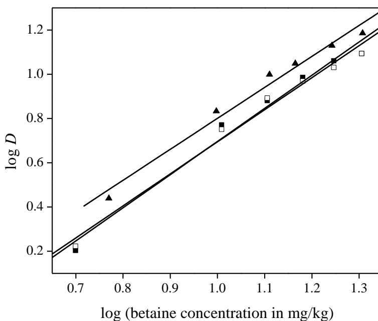
Figure 10. Slope analysis for the extraction of neodymium from chloride (■), nitrate (□) and bis(trifluoromethylsulfonyl)imide (▲) feed solution in [\text{Hbet}][\text{Tf}_2\text{N}]-\text{H}_2\text{O} with zwitterionic betaine as extractant. The slope of linear fit is equal to 1.50 \pm 0.10 (■), 1.40 \pm 0.10 (□), 1.45 \pm 0.09 (▲), respectively.
