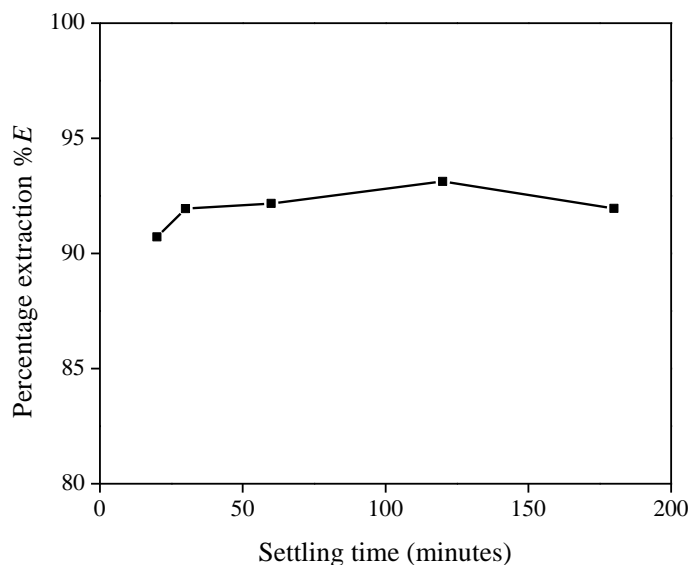
Figure 6. Percentage extraction (% E ) as a function of the settling time (in minutes) for the extraction of \text{Nd}(\text{Tf}_2\text{N})_3 in [\text{Hbet}][\text{Tf}_2\text{N}]-\text{H}_2\text{O} with betaine as extractant.
