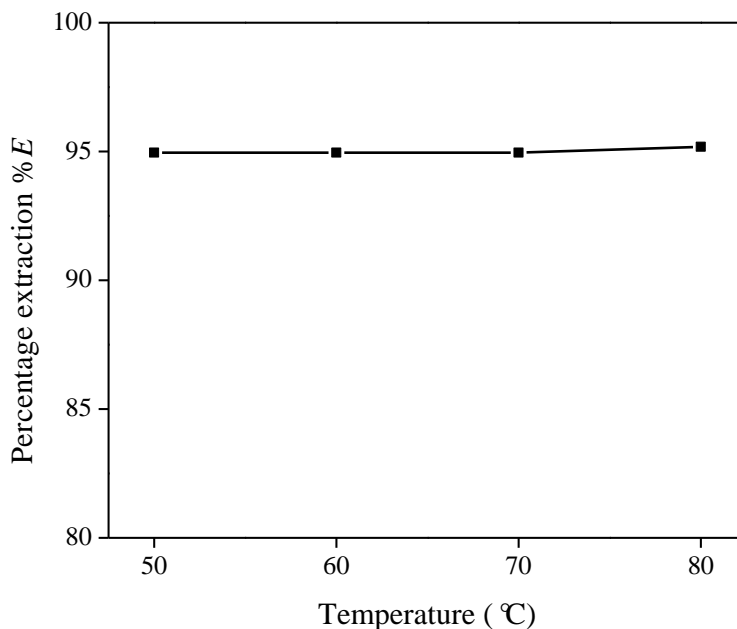
Figure 4. Percentage extraction (% E ) as a function of the temperature of the homogeneous stage for the extraction of Nd(Tf 2 N) 3 in [Hbet][Tf 2 N]–H 2 O with betaine as extractant.
