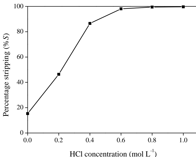
Figure 13. Percentage stripping (%S) as a function of different HCl concentrations for the stripping neodymium from [Hbet][Tf 2 N].
